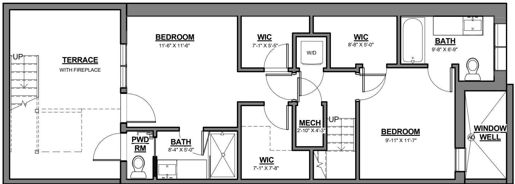
BEDROOM FLOOR
