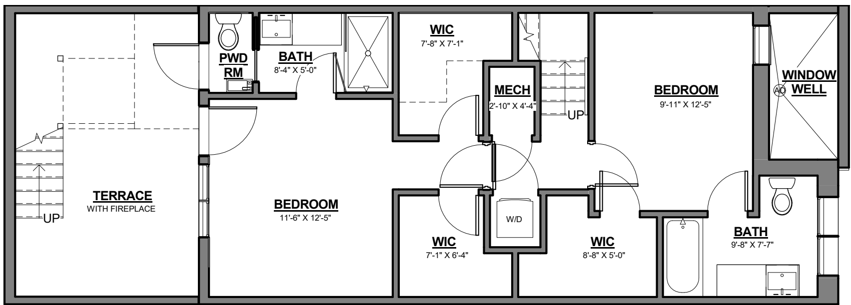
BEDROOM FLOOR
