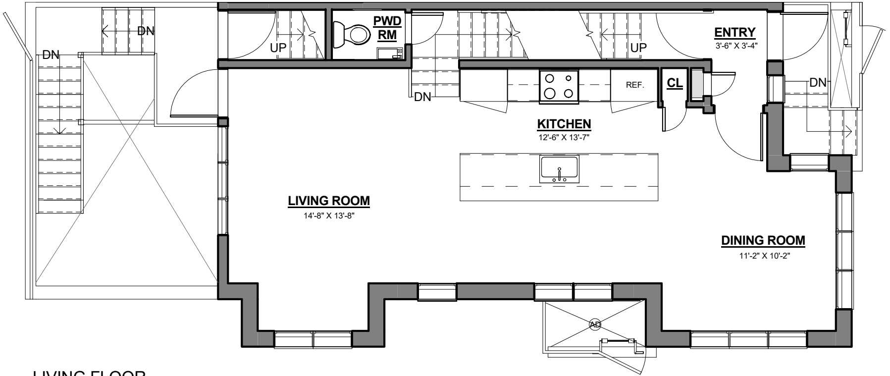
LIVING FLOOR
