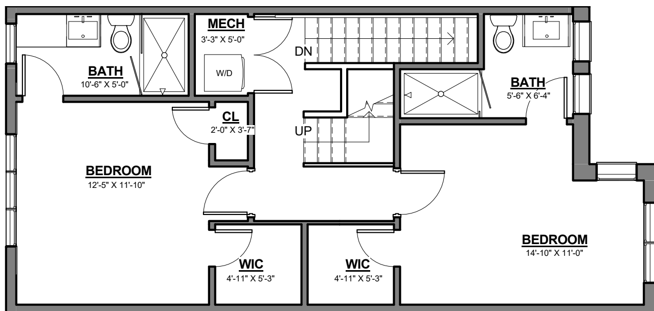
BEDROOM FLOOR
