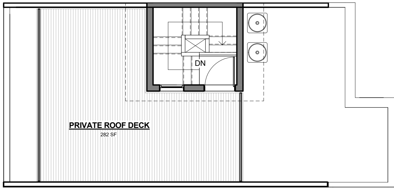
ROOF DECK
