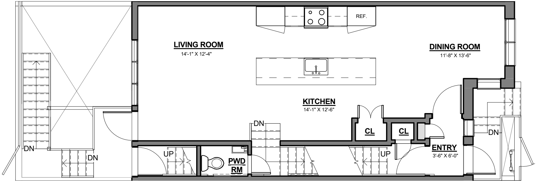
LIVING FLOOR
