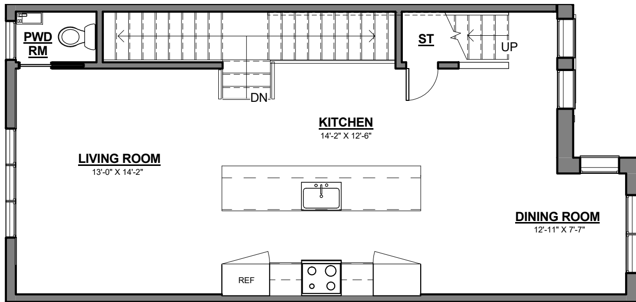
LIVING FLOOR
