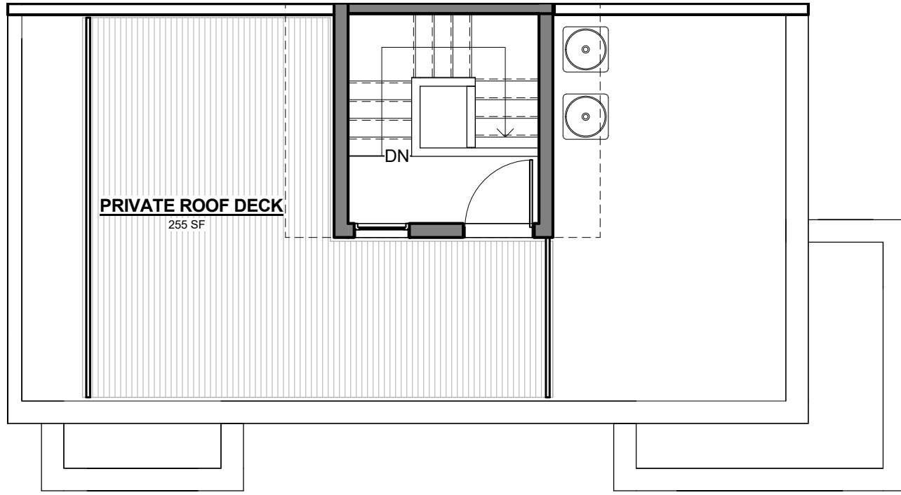
ROOF DECK
